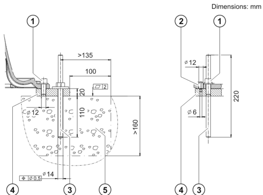
Fig. 6-3: Cross-section of foundations
