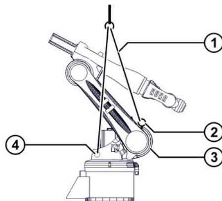
Fig. 7-4: Lifting tackle
