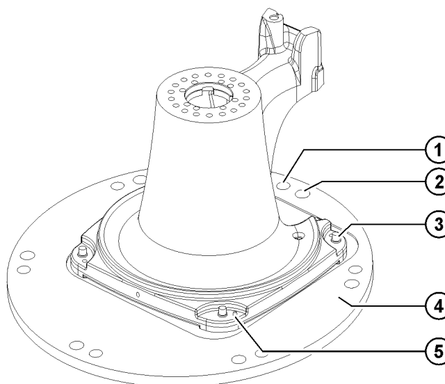
Fig. 6-6: Adapter plate
