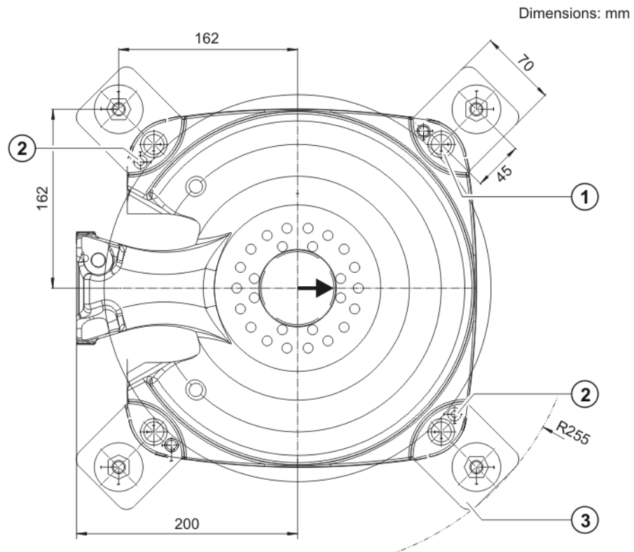
Fig. 6-2: Mounting base with centering, dimensioned drawing
